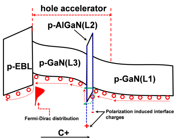
FIG. 1. Schematic energy diagram of the proposed accelerator. Solid green arrow and dashed green one illustrate the hole transport through intraband tunneling and thermionic emission, respectively.
