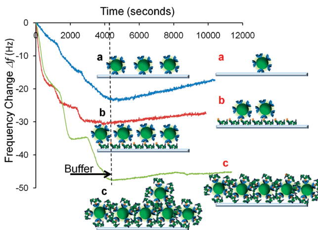
Figure 3. QCM-D real-time monitoring of the binding of SA-QDs for (a) the control set, (b) the sequential assembly set, and (c) the hybrid nanoassembly set on silica surface.
