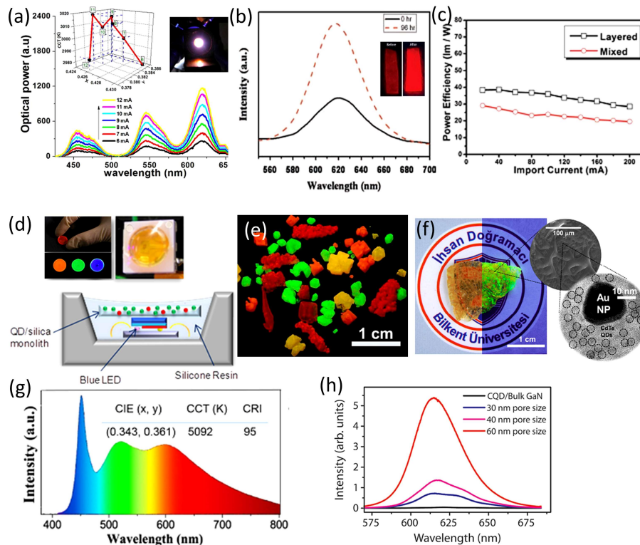
Figure 1: (a) Spectrum of the quantum dot (QD)-integrated white light-emitting diode (LED) exhibiting a color rendering index (CRI) ~90, luminous efficiency of the optical radiation (LER) = 357 \text{lm/W}_{opt} , and correlated color temperature (CCT) = 2982 K. Reproduced with permission from Ref. [10], Copyright Optical Society of America. (b) Photoluminescence of the red-emitting QDs embedded within silicone before (black curve) and after (red curve) ultraviolet (UV) treatment along with the real-color photographs of their films under UV illumination before and after the UV treatment (inset). Reproduced with permission from Ref. [19], Copyright Wiley International. (c) Luminous efficiency (also known as power efficiency) of the white LEDs produced by applying layered QD architecture (black) and mixed QD architecture (red) on a blue LED. Reproduced with permission from Ref. [22], Copyright Royal Society of Chemistry. (d) Illustration of the white LED produced using silica monolith along with the single color QD incorporated silica monoliths and the real-color photograph of the white LED. Reproduced with permission from Ref. 26, Copyright American Chemical Society. (e) Real-color photographs of the QD-embedded salt macrocrystals under UV illumination. Reproduced with permission from Ref. [29], Copyright American Chemical Society. (f) Real color- photograph of QD and Au NP co-immobilized macrocrystals exhibiting fluorescence enhancement under ambient lighting and UV illumination along with their scanning electron microscopy and transmission electron microscopy images. Reproduced with permission from Ref. [30], Copyright Tsinghua University Press and Springer-Verlag Berlin. (g) Emission spectrum of the Cu and Mn-doped QD integrated white LED. Reproduced with permission from Ref. [31], Copyright American Chemical Society. (h) Emission spectrum of the red-emitting QDs placed on bulk and porous GaN surface with varying pore sizes. Reproduced with permission from Ref. [32], Copyright Wiley International.
