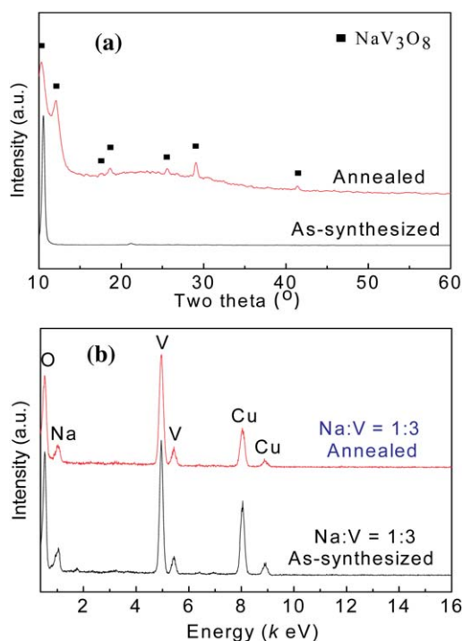
Fig. 1 (a) XRD patterns of the as-synthesized nanobelts and the annealed nanobelts at 400 °C in air and (b) EDS spectra of the as-synthesized nanobelts and the annealed nanobelts at 400 °C in air.
