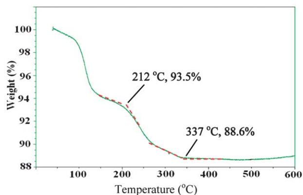
Fig. 2 TGA curve of the as-synthesized nanobelts measured in air with a heating rate of 10 °C min ^{-1} .
