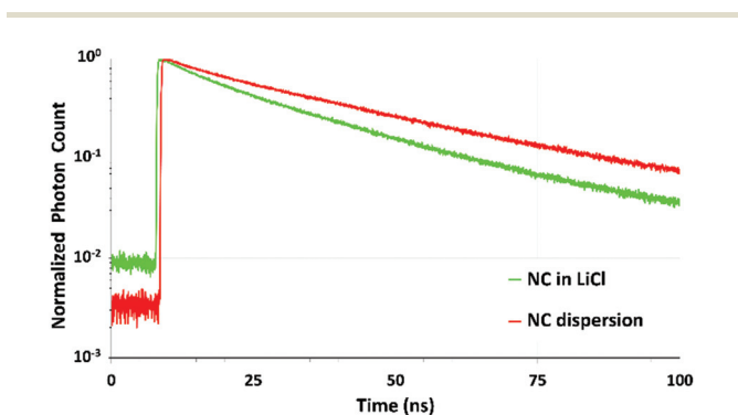
Fig. 3 Time-resolved photoluminescence decay curves of the NCs in dispersion and the same NCs encapsulated in LiCl.
