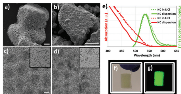
Fig. 2 Scanning electron microscopy (SEM) images of the LiCl powders (a) without and (b) with NCs (scale bars: 30 \mu\text{m} ). Transmission electron microscopy (TEM) images of (c) the as-synthesized NC dispersion in hexane and (d) the NC-in-LiCl powders (scale bars of larger images: 5 nm and inset images: 50 nm). (e) Photoluminescence spectra of the nonpolar NCs in dispersion and the same NCs encapsulated within LiCl ionic salt. Also, absorption spectra of the as-synthesized NCs (dispersion in hexane) and NC-in-LiCl powder film were provided. Real colour photographs of the LiCl encapsulated NC film under (f) ambient lighting and (g) UV illumination at 366 nm.
