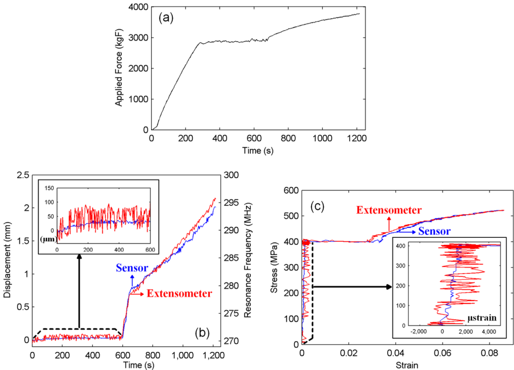
Figure 3.7: Plastic region strain and displacement measurements: a) The applied force, b) Displacement data from the sensing system compared to the extensometer data. Corresponding resonance frequencies of the sensor are also given on the right vertical axis. Top left: Zoomed elastic region (inset), c) Stress versus strain acquired from the sensor and from the extensometer. Bottom right: Zoomed elastic region (inset). (Reprinted, with permission, from “Wireless Measurement of Elastic and Plastic Deformation by a Metamaterial-Based Sensor” by B. Ozbey, H. V. Demir, O. Kurc, V. B. Erturk and A. Altintas, Sensors , under the Creative Commons Attribution License ( http://creativecommons.org/licenses/by/4.0/ ).)
