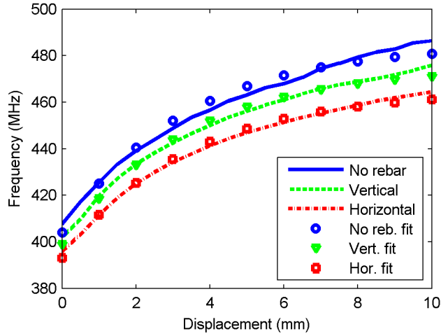
Figure 4.9: Translation stage measurements of the change of the sensor resonance frequency with d at the no-rebar case and for the cases of vertical and horizontal placement of the rebar grid fragment behind the NSRR probe, shown along with the exponential fits for each case. l = 2 cm in all cases.
